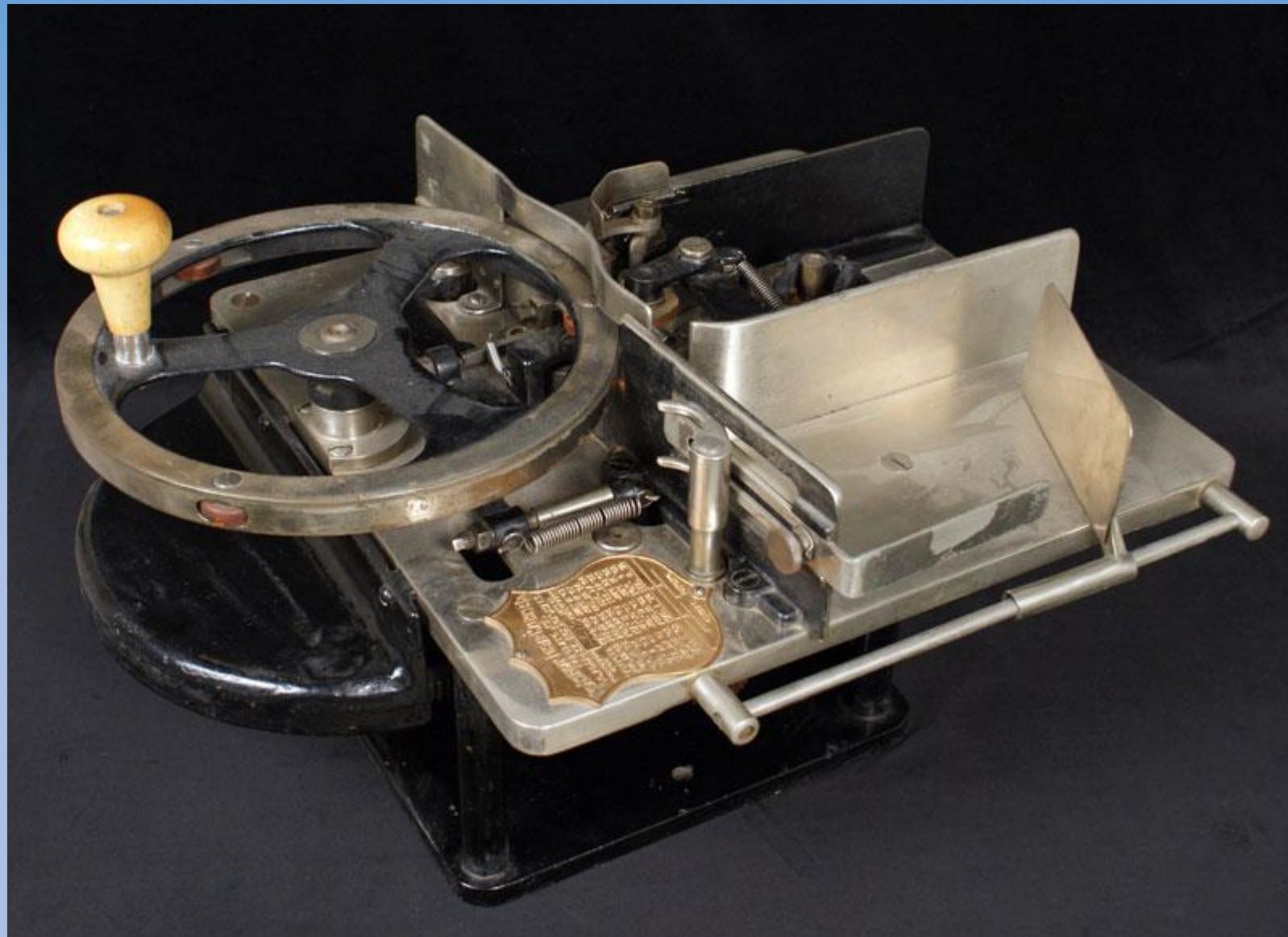
American Postal Machines Company stamp canceling machine 1900-1920
