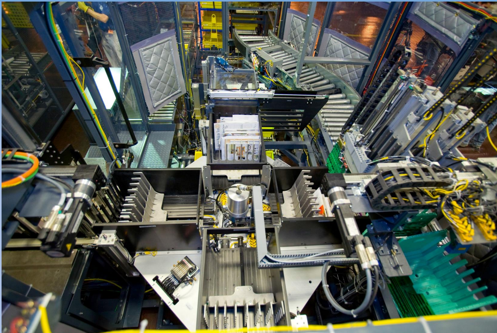
Flat Sequencing System (FSS)
