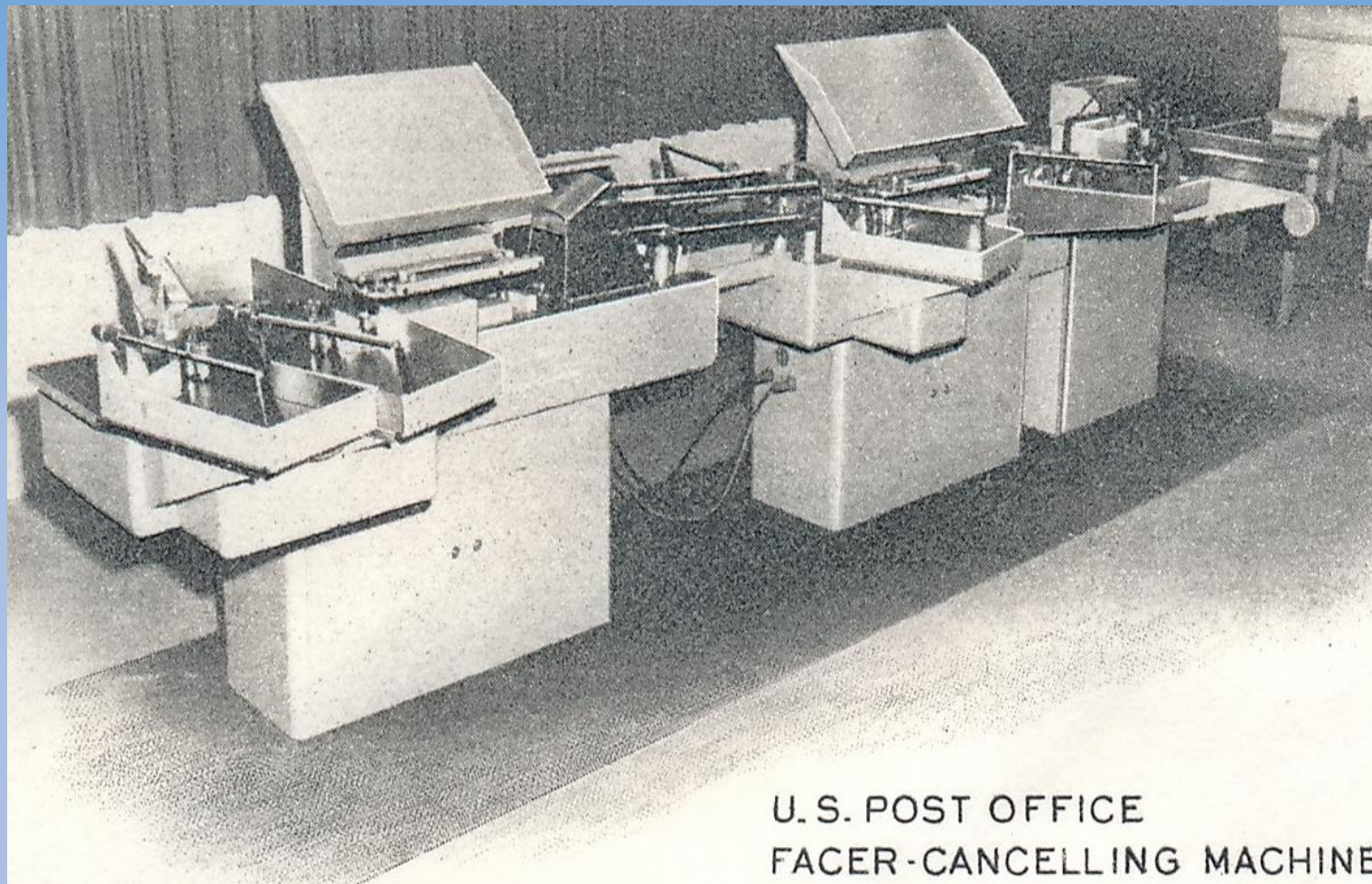
Pitney-Bowes Mark II (Dayton, OH)
