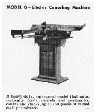
Afb. 5 Model G - Electric Cancelling Machine
